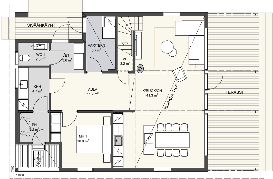
1. krs
