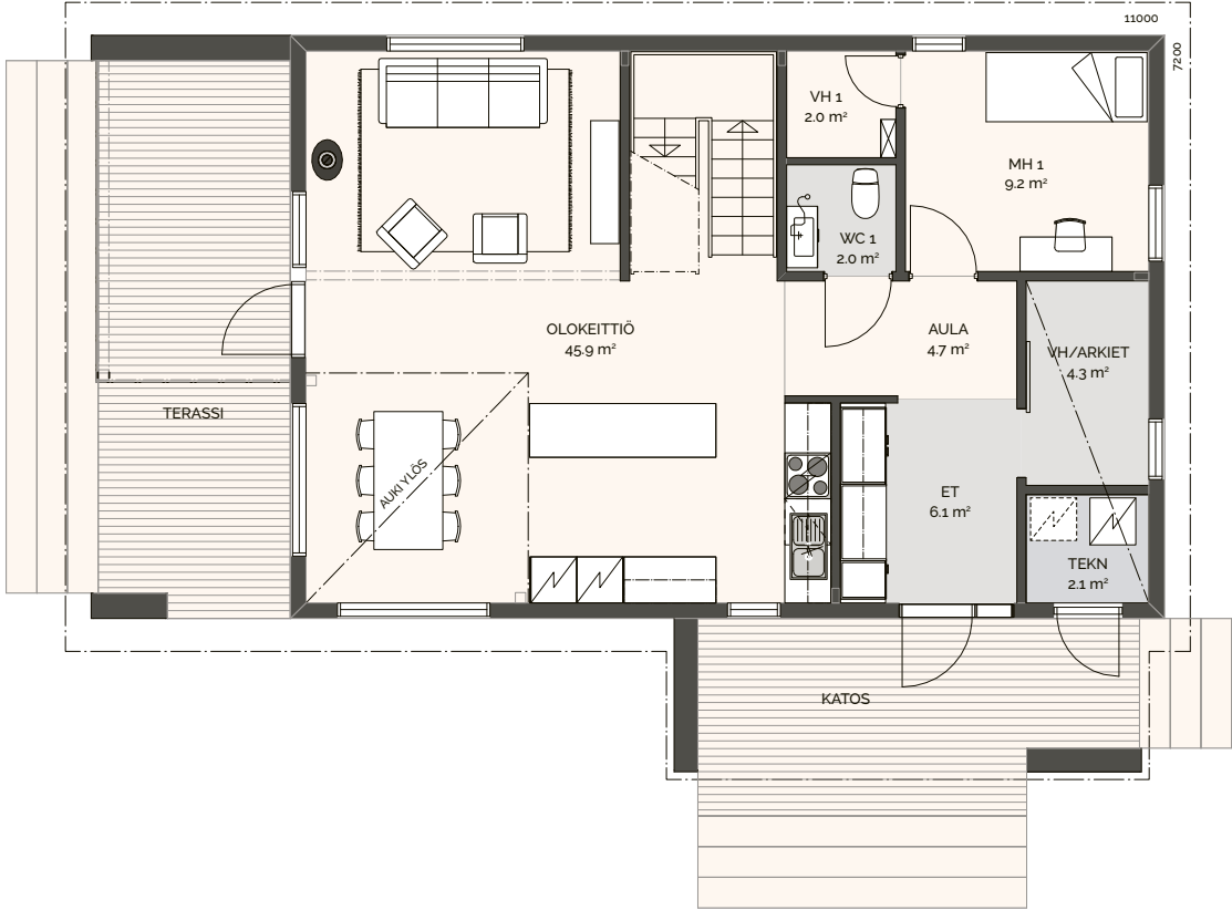
1. krs
